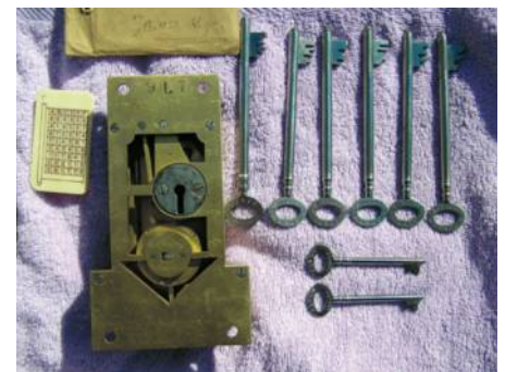
Note the Steel hardened keyhole surround, a standard Chatwood Invincible design feature protecting against drill and other keyhole damage.
